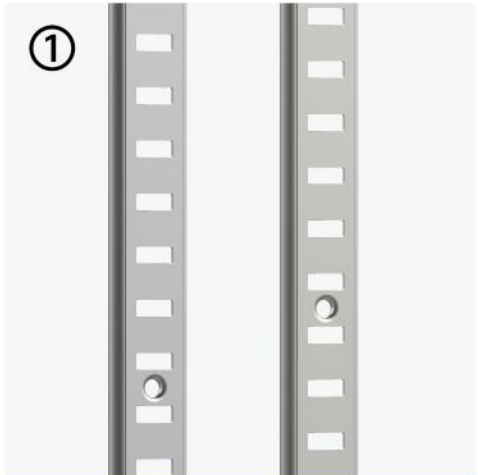
① 支撑条 20x4.1 - 铝款(左) / 不锈钢款(右) Din Rail - Aluminum(L) / Stainless Steel(R)
